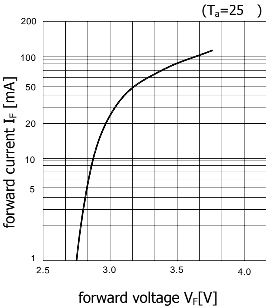
(1) forward voltage vs. forward current
